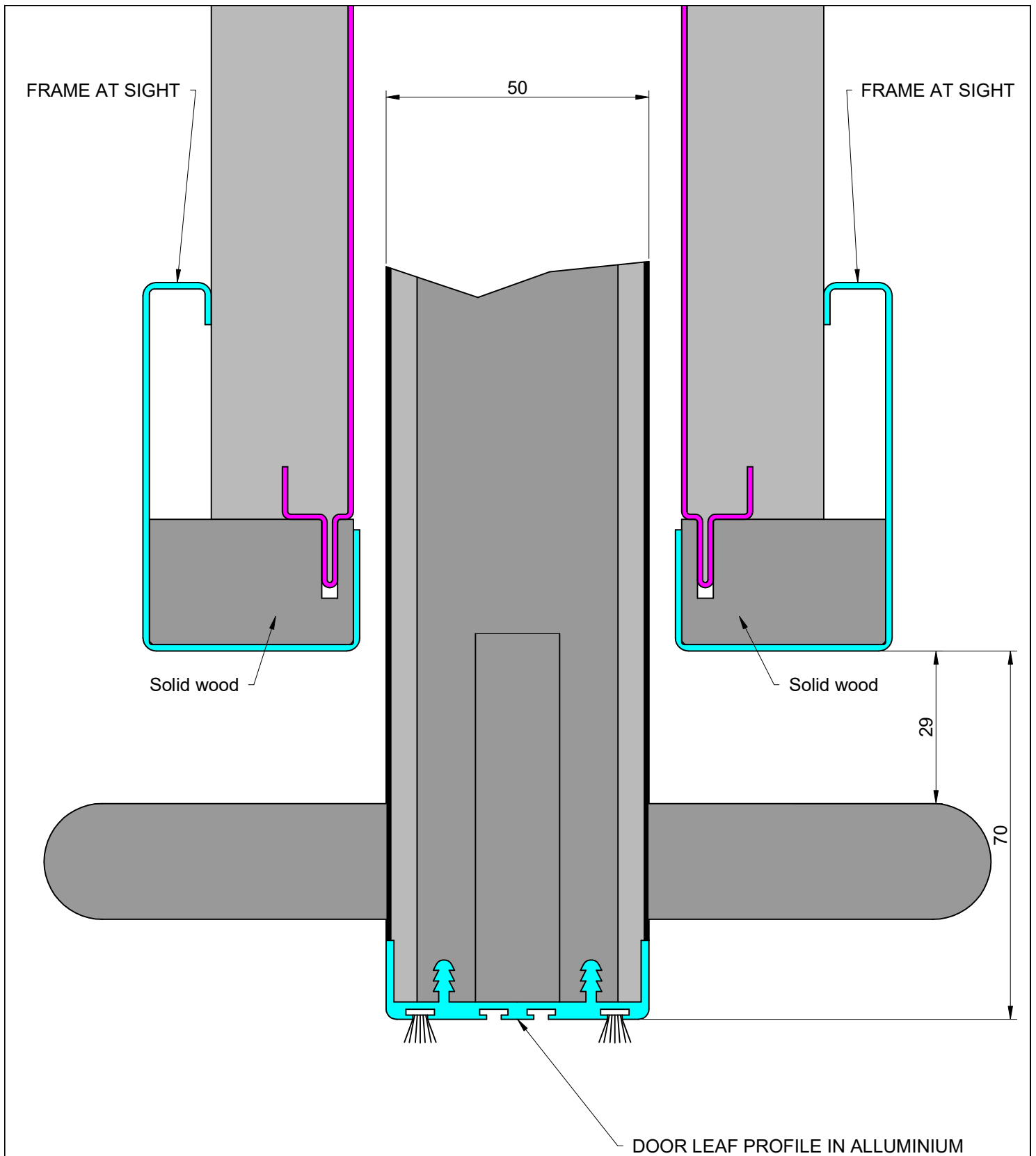
Internal sliding door squared frame (ray 2,5 mm)
