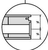
Lock side for thickness door leaf 30+38 mm
